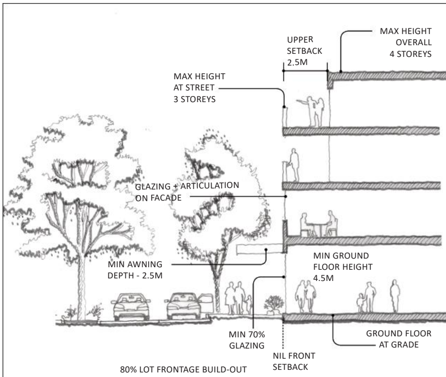
Figure 1 FRONTAGE TYPE 1
