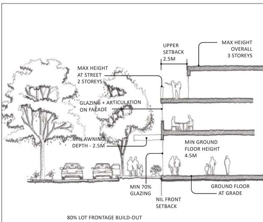
Figure 2 FRONTAGE TYPE 2
