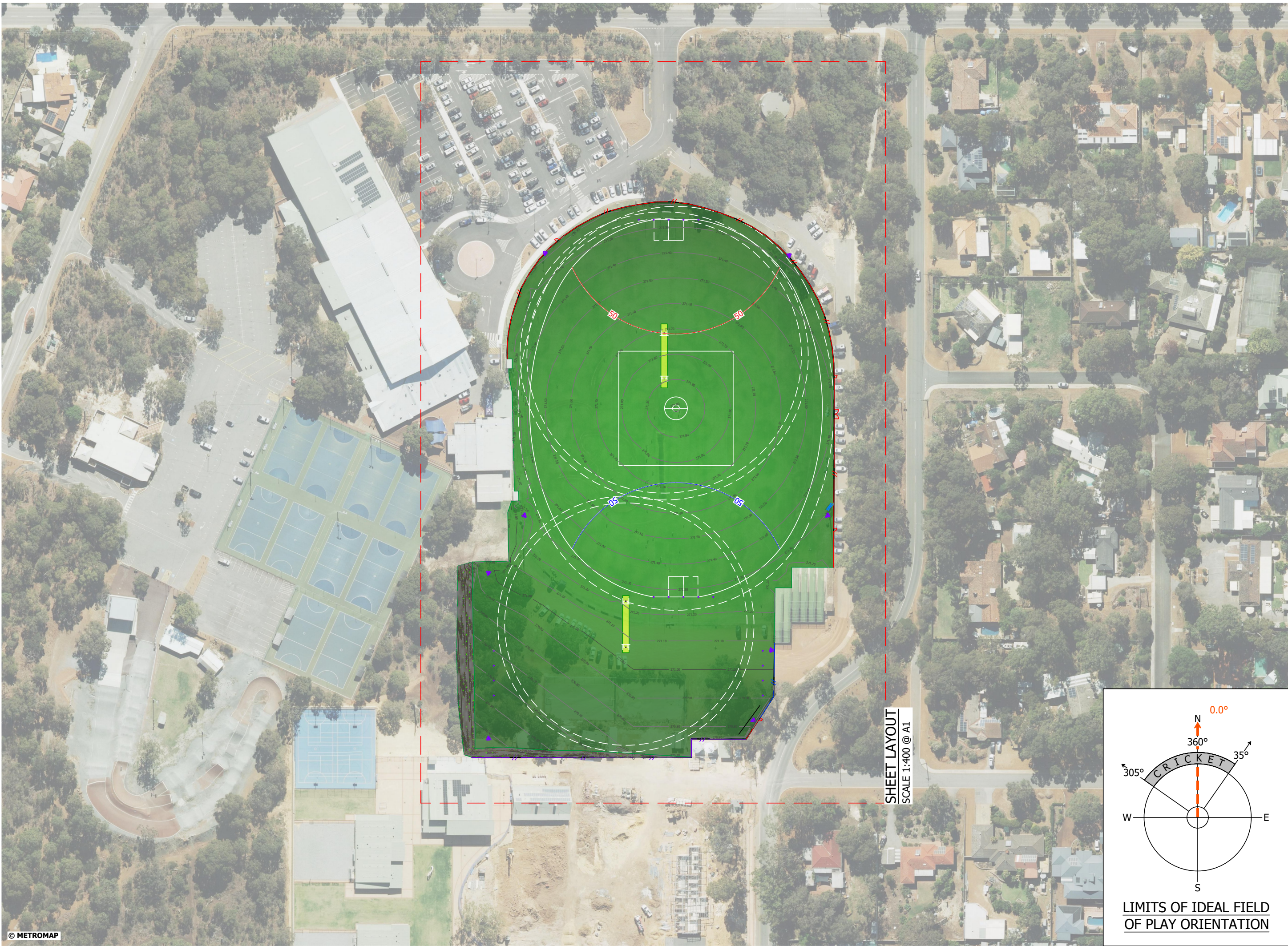
OVERALL SITE LAYOUT PLAN ALL AERIAL IMAGERY USED IN THE PRODUCTION OF THIS DRAWING SET HAVE BEEN UNDER LICENSE FROM METROMAP.
