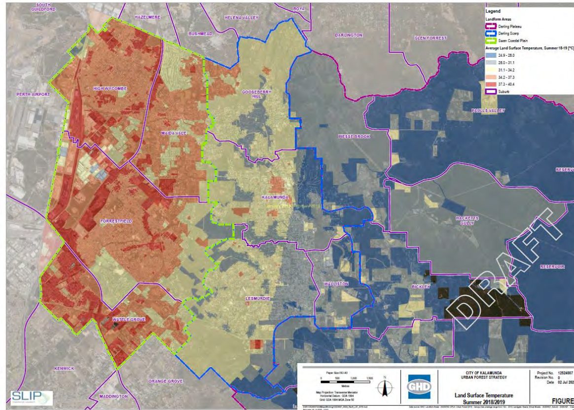
Figure 5 Urban heat island effect, GHD 2020
